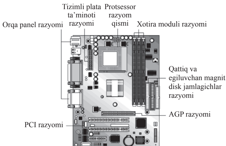
2.5-rasm. Micro-ATX standartli tizimli plata.
