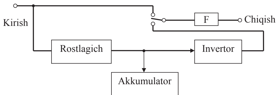
11.8-rasm. Ikki barobar o‘zgartirgichli UPS ning blok-sxemasi (on-line).
