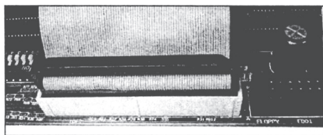
3.9-rasm. Tizimli plataga IDE shleyfining ulanishi.
