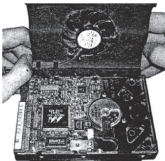
3.16-rasm. Vinchesterga sovitish qurilmasini o'rnatish.
