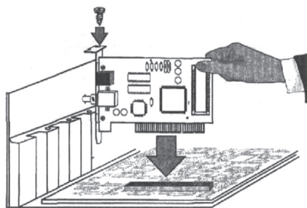
8.8-rasm. Tarmoq adapterini tizimli platadagi razyomga o‘rnatish.
