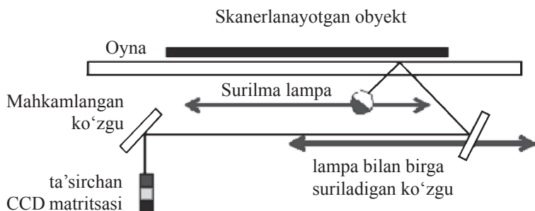
4.8-rasm. Skaner ishlashining sxematik ko‘rinishi
