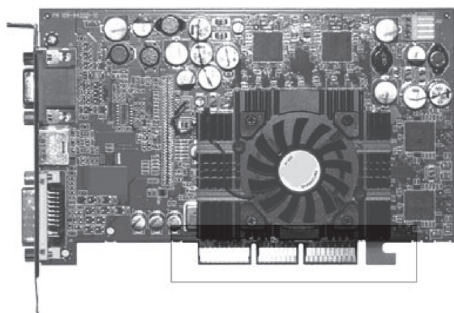
7.4-rasm. Videokartaning interfeys qismi.
