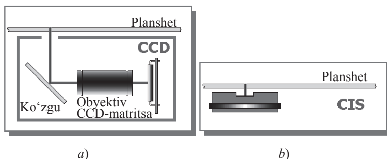
4.9-rasm. Oynali tizim: CCD-skaner (a), CIS-skaner (b).
